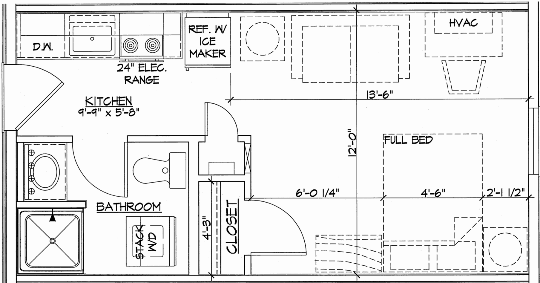
EFFICIENCY UNIT FLOOR PLAN
