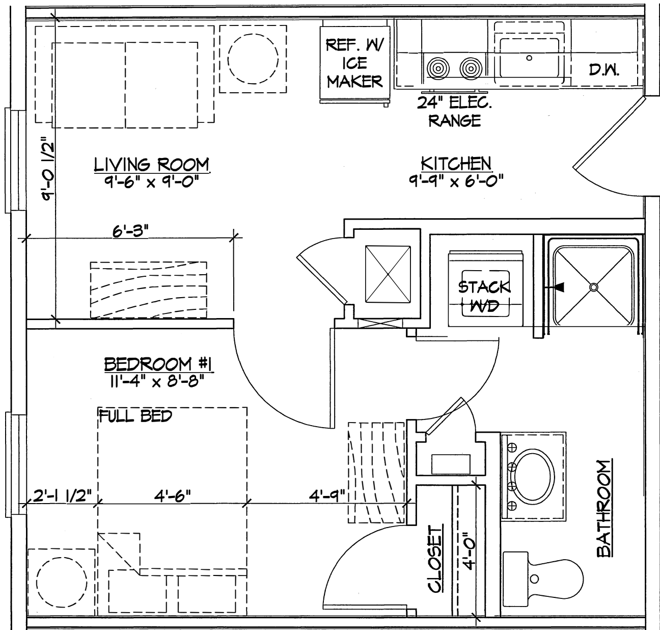
1 BEDROOM UNIT FLOOR PLAN
