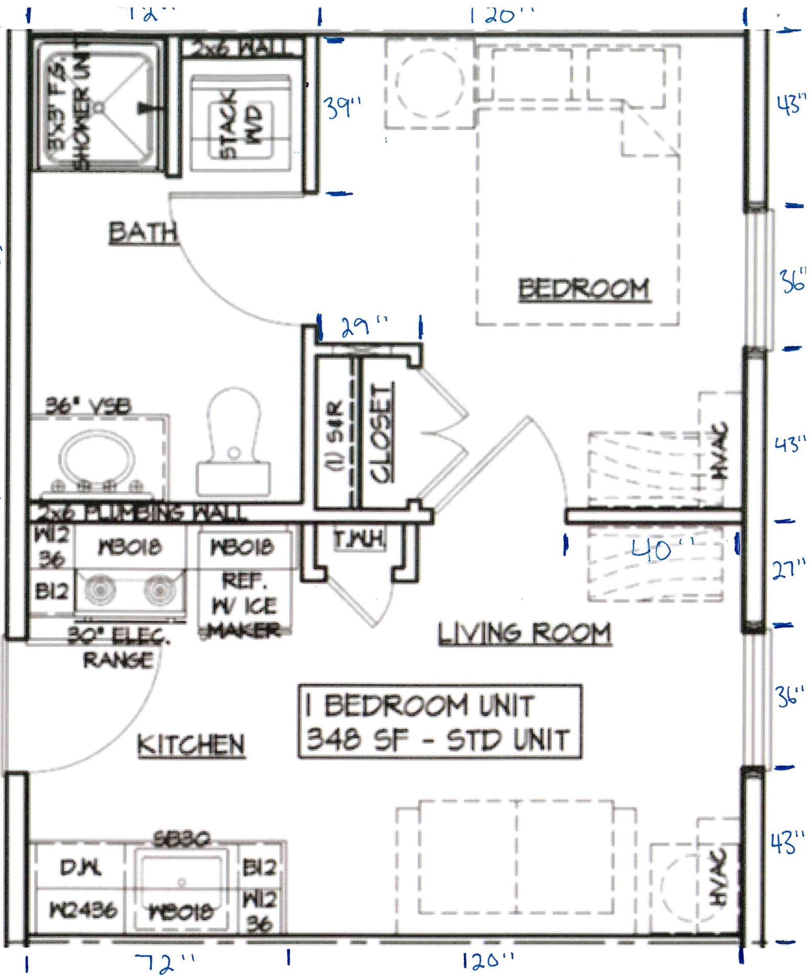
One Bedroom Layout
